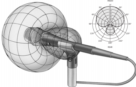
Supercardioid Microphone
